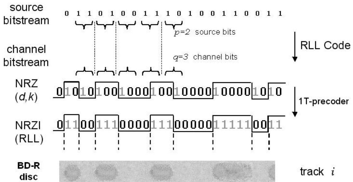
Figure 3.1.2: RLL d=1 coding for BD optical recording.
