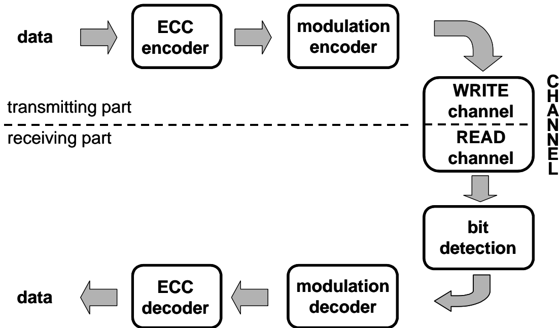
Figure 3.1.1: Schematic form of a digital storage system.
