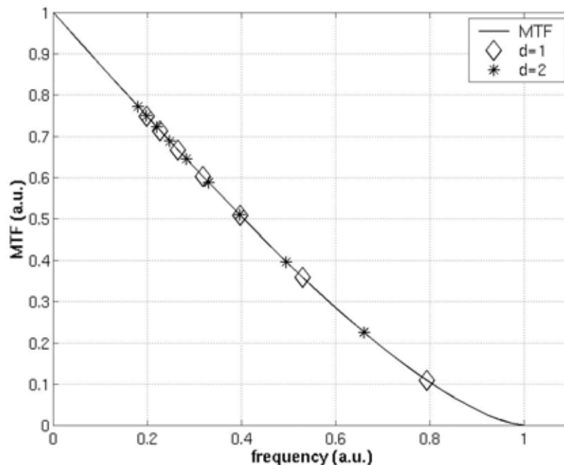
Figure 3.1.3: MTF for the optical recording channel as a function of frequency (in arbitrary units, with the cut-off at "1") with the frequencies of the pure tones ... |nT_d| |nT_d| ... superimposed.
