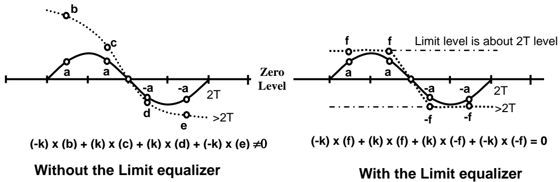
Fig.2.5.3 Behavior of Linear EQ and Limit-EQ
