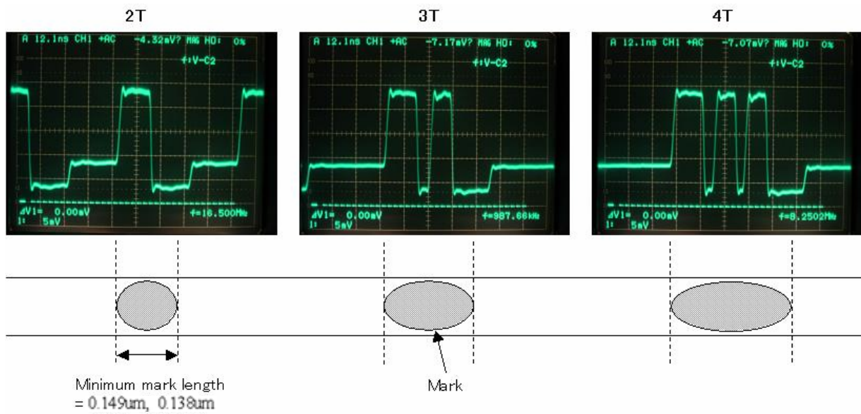
Fig. 2.2.3 Write Pulse Waveform
