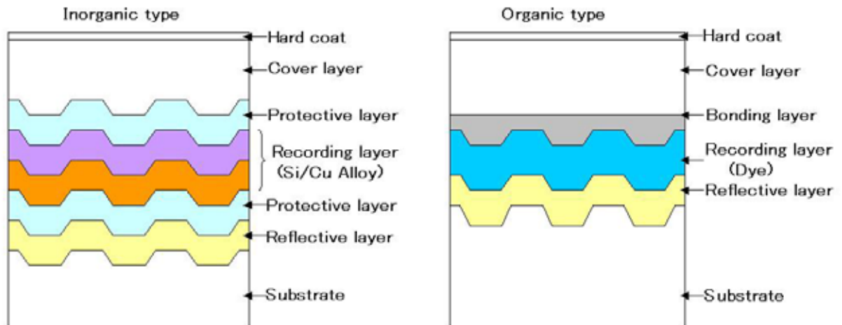
Fig. 2.2.2 Disc structure
