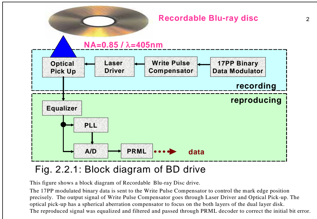
Fig. 2.2.1 Basic recording/playback system of BD-R
