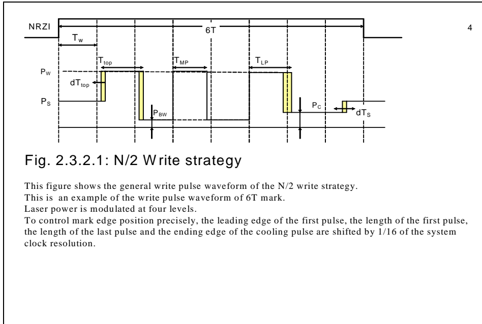
Fig. 2.3.2.1 N/2 write strategy
