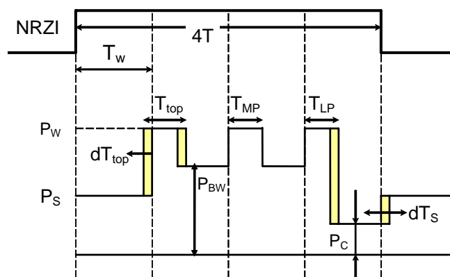
Fig. 2.3.1.2 N-1 Write strategy power levels
