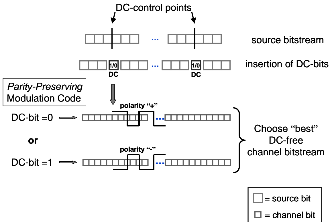
Figure 3.1.5: Principle of DC-control via parity-preserving modulation code.
