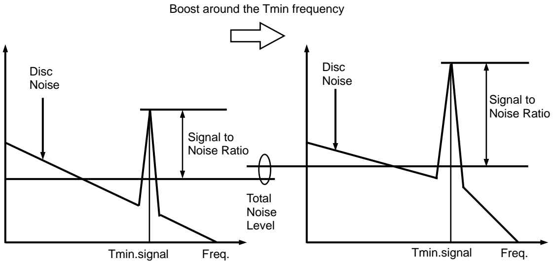
Fig. 2.5.1 S/N improvement by the high frequency boost
