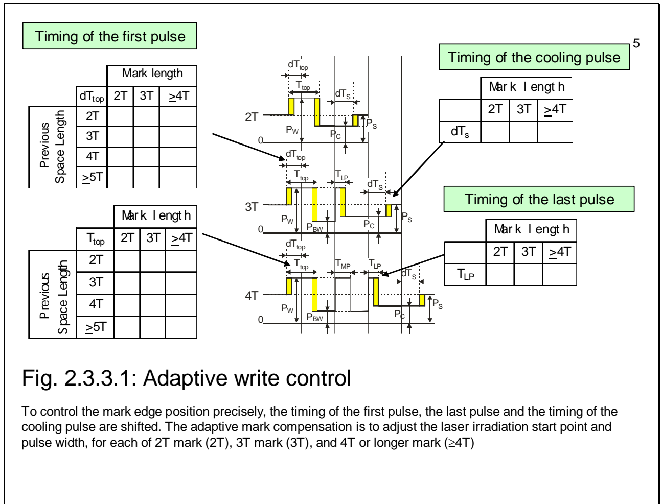
Fig. 2.3.3.1 Adaptive write control
