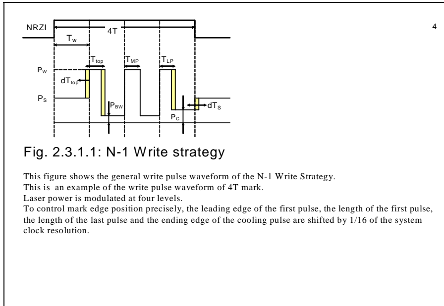
Fig. 2.3.1.1 N-1 Write strategy
