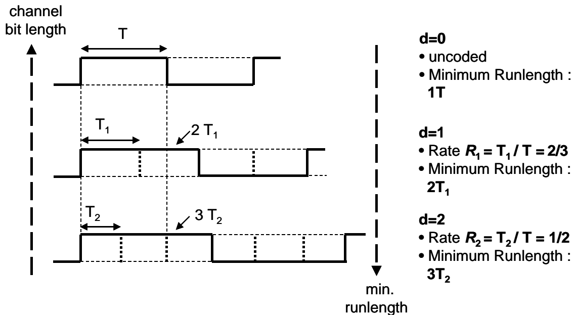
Figure 3.1.4 Channel bit length and minimum runlength for different d constraints at the same recording capacity.
