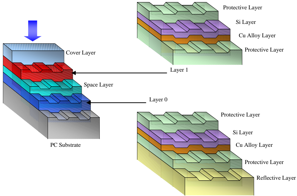
Figure 2.6.3 Cross section of TDK's dual-layer BD-R disc.
