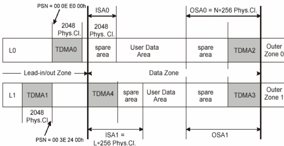
Fig 5.1.1. Location of the TDMAs on the disc
